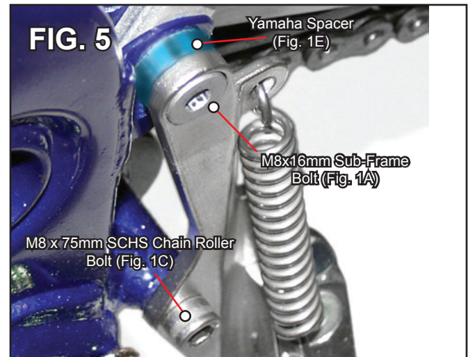
2005 YZ250F/YZ450F Kickstand Bracket Installed
